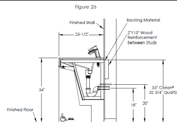
Rough-In (Four Station); Section View
