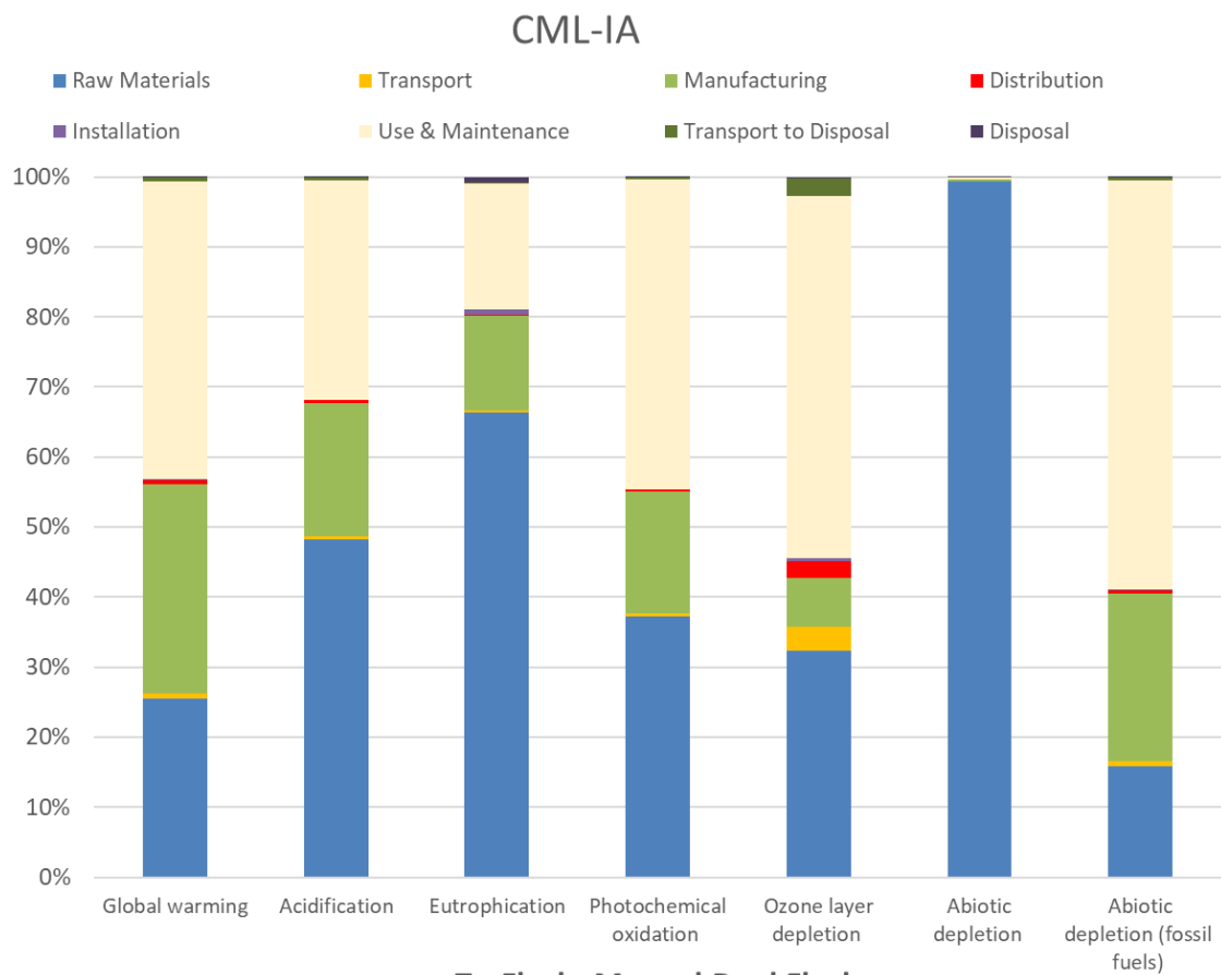
Figure 4. Contribution analysis for the Sloan TruFlush Manual Dual Flush flushometer – CML-IA. (excluding product replacements (B4) and operational water use (B7)).
